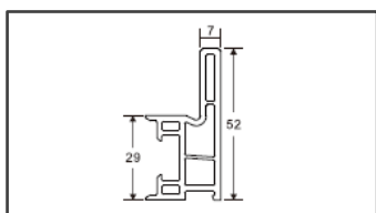
Mesh Adapter Code: D067 Weight (kg/m): 0.54 Pcs/Bag : 20
