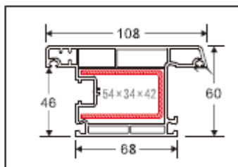
Out-Swing Opening Door Sash Code: D003 Weight (kg/m): 1.55 Pcs/Bag : 4
