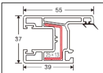
55mm Sash with Gasket Code: D102 Weight (kg/m): 0.75 Pcs/Bag : 8
