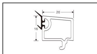
Casement 20mm Glass Bead Code: FUx009 Weight (kg/m): 0.220 Pcs/Bag : 30
