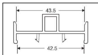
Sash Connector Code: D061 Weight (kg/m): 0.285 Pcs/Bag : 20
