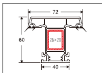
T Mullion with Gasket Code: D004 Weight (kg/m): 1.1 Pcs/Bag : 6
