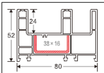
2.5 Track Sliding frame Code: D101 Weight (kg/m): 1.135 Pcs/Bag : 6
