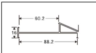
60mm/90mm Coupler Code: D021 Weight (kg/m): 0.26 Pcs/Bag : 15
