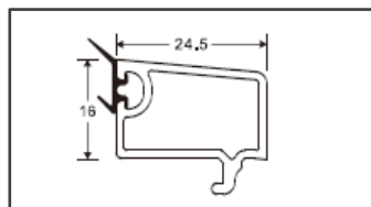
Sliding 5mm Glass Bead Code: D059 Weight (kg/m): 0.25 Pcs/Bag : 20
