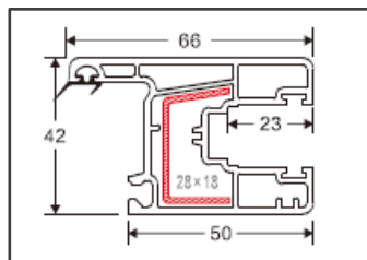
66mm Sash with Gasket Code: D054G Weight (kg/m): 1.0 Pcs/Bag : 4
