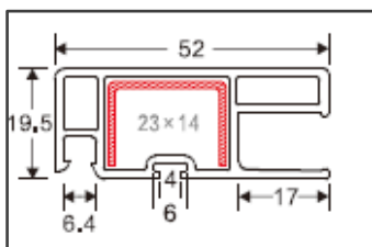
Sliding Window Mesh Sash Code: D056W Weight (kg/m): 0.495 Pcs/Bag : 15
