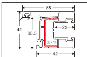
58mm Sash with Gasket Code: D062G Weight (kg/m): 0.87 Pcs/Bag : 8
