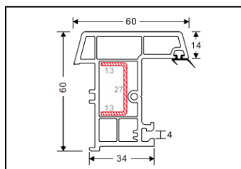
Fly Mullion Code: D005 Weight (kg/m): 1.035 Pcs/Bag : 6
