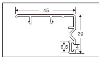
Window Sash Interlock Code: D057 Weight (kg/m): 0.21 Pcs/Bag : 30
