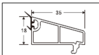
Casement 5mm Glass Bead Code: D008 Weight (kg/m): 0.3 Pcs/Bag : 20
