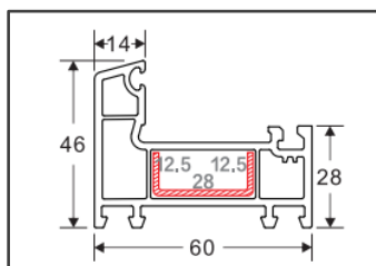
Casement Frame Small Code: D001S Weight (kg/m): 0.81 Pcs/Bag : 6
