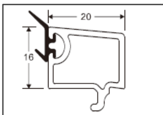
Sliding 5mm Glass Bead Code: D105 Weight (kg/m): 0.22 Pcs/Bag : 30
