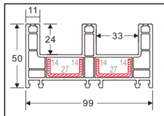
3 Track Sliding frame 99mm Code: FUx108 Weight (kg/m): 1.5 Pcs/Bag : 4
