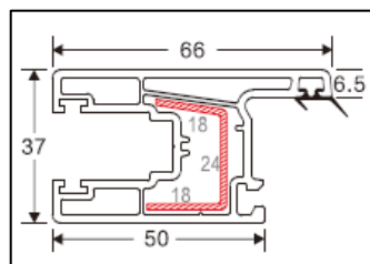
66mm Sash with Gasket Code: D103 Weight (kg/m): 0.87 Pcs/Bag : 8
