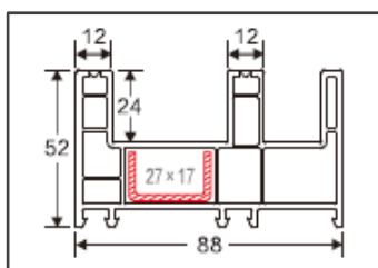
2.5 Track Sliding frame Code: D052A Weight (kg/m): 1.19 Pcs/Bag : 6
