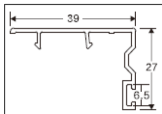
Sash Interlock Code: D104 Weight (kg/m): 0.18 Pcs/Bag : 30
