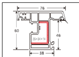
Out-Swing Opening Window Sash Code: D002 Weight (kg/m): 1.15 Pcs/Bag : 6
