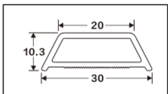
30mm Grill Outlay Code: D069 Weight (kg/m): 0.15 Pcs/Bag : 30
