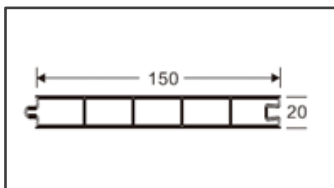
Door Panel Code: D015 Weight (kg/m): 0.9 Pcs/Bag : 8
