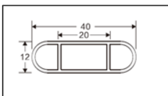
Louver Blade Code: D018 Weight (kg/m): 0.21 Pcs/Bag : 20
