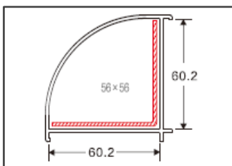
90 deg Bay Pole Code: D013 Weight (kg/m): 0.71 Pcs/Bag : 4
