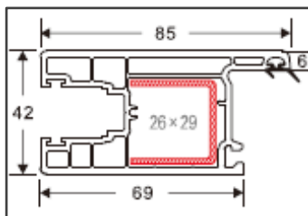
85mm Sash with Gasket Code: D055G Weight (kg/m): 1.2 Pcs/Bag : 4
