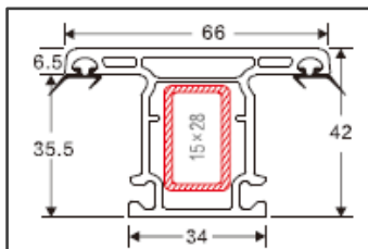
Sliding Sash Mullion Code: D063 Weight (kg/m): 0.84 Pcs/Bag : 8
