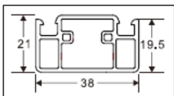
Mesh Sash Mullion Code: D065 Weight (kg/m): 0.35 Pcs/Bag : 15
