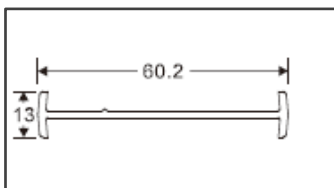
60mm/60mm Coupler Code: D011 Weight (kg/m): 0.24 Pcs/Bag : 20
