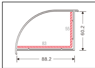
88 - 60 Bay Corner Code: D014 Weight (kg/m): 0.89 Pcs/Bag : 4
