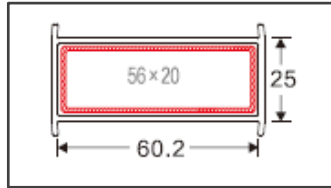
Box Coupler Profile Code: D012 Weight (kg/m): 0.59 Pcs/Bag : 6
