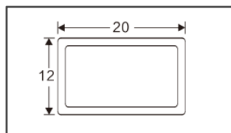
20mm Grill Code: D068 Weight (kg/m): 0.12 Pcs/Bag : 20
