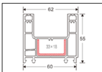
2 Track Sliding frame Code: D051 Weight (kg/m): 1.02 Pcs/Bag : 6
