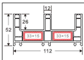
3 Track Sliding frame Code: D053 Weight (kg/m): 1.625 Pcs/Bag : 4
