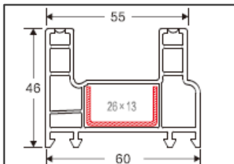
2 Track Sliding frame Code: D107 Weight (kg/m): 0.82 Pcs/Bag : 6
