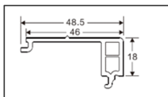
Louver Shutter Bead Code: D019 Weight (kg/m): 0.24 Pcs/Bag : 20
