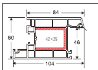
In-swing Door Sash Code: D007 Weight (kg/m): 1.45 Pcs/Bag : 4
