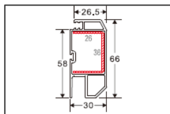
Sliding Door Mesh Sash Code: D056D Weight (kg/m): 0.59 Pcs/Bag : 9
