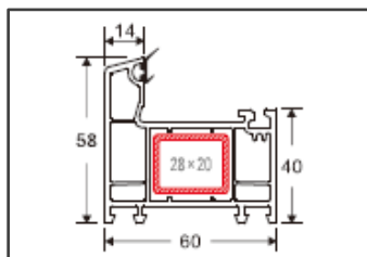
Casement Frame with Gasket Code: D001G Weight (kg/m): 0.98 Pcs/Bag : 6
